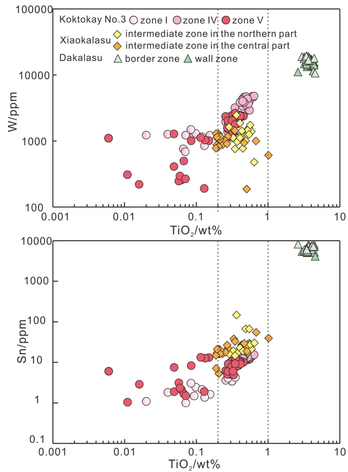
Fig. S1. Plots of \text{TiO}_2 vs. W and \text{TiO}_2 vs. Sn.
